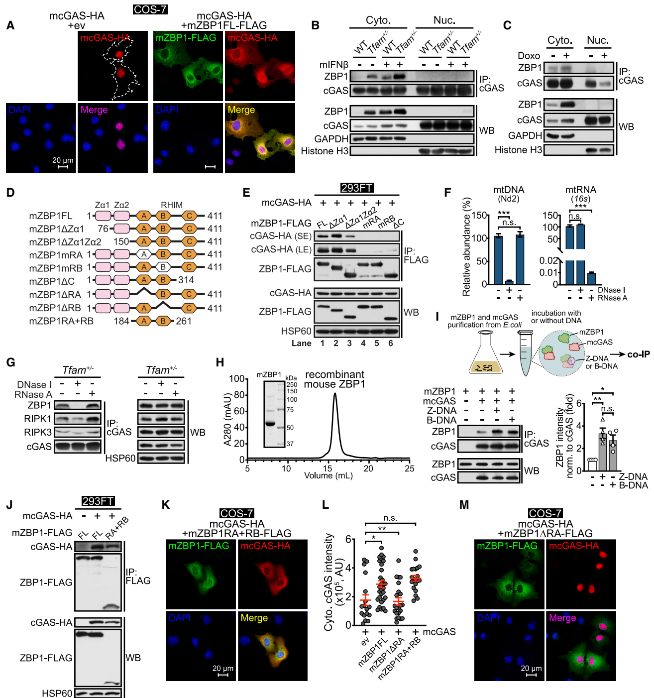
Figure 3. ZBP1 binds to cGAS in a DNA- and RHIM-dependent manner
