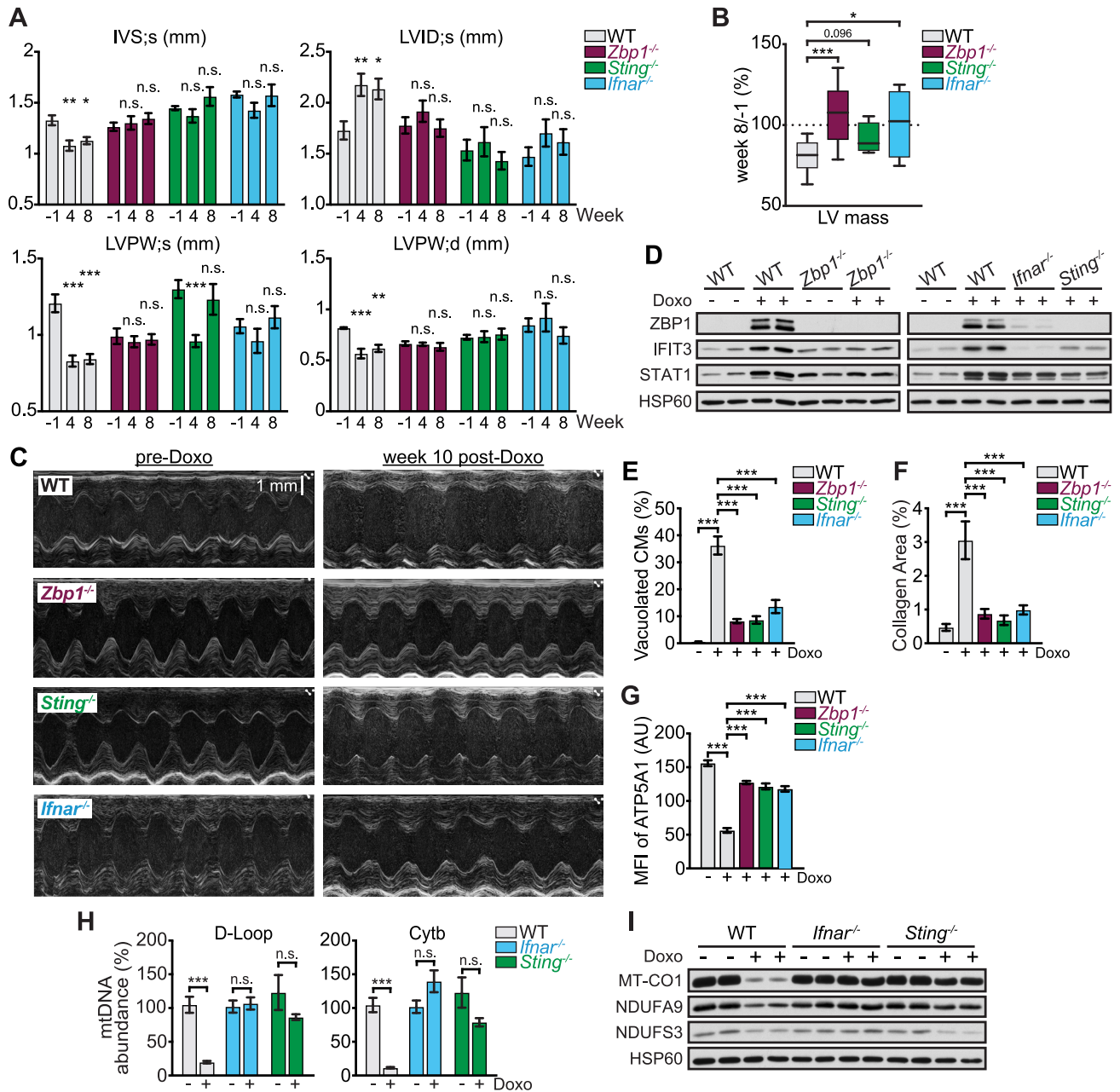
Figure S7. Doxorubicin-induced ISG expression and cardiac dysfunction are lessened in the absence of ZBP1-STING-IFNAR signaling, related to Figure 7
